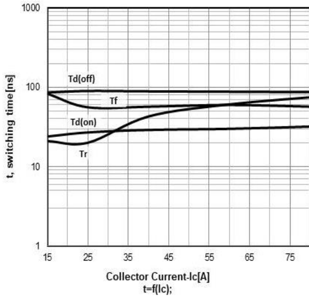
Switching times vs collector current T_j=25\text{ }^{\circ}\text{C}
