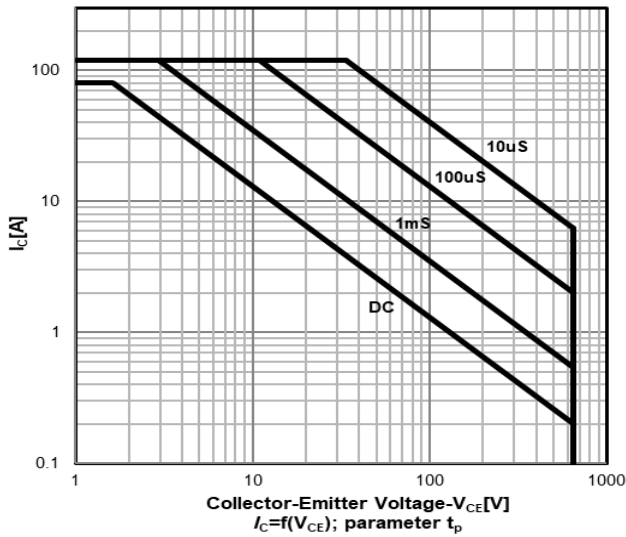
Safe operating area T_a=25^\circ\text{C} Non-Full PAK
