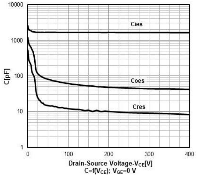
Capacitance characteristics
