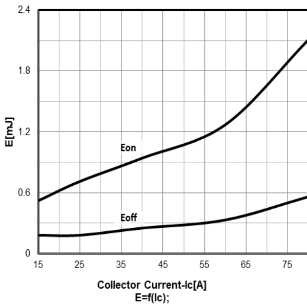
Switching energy losses vs collector current T_j=25\text{ }^{\circ}\text{C}
